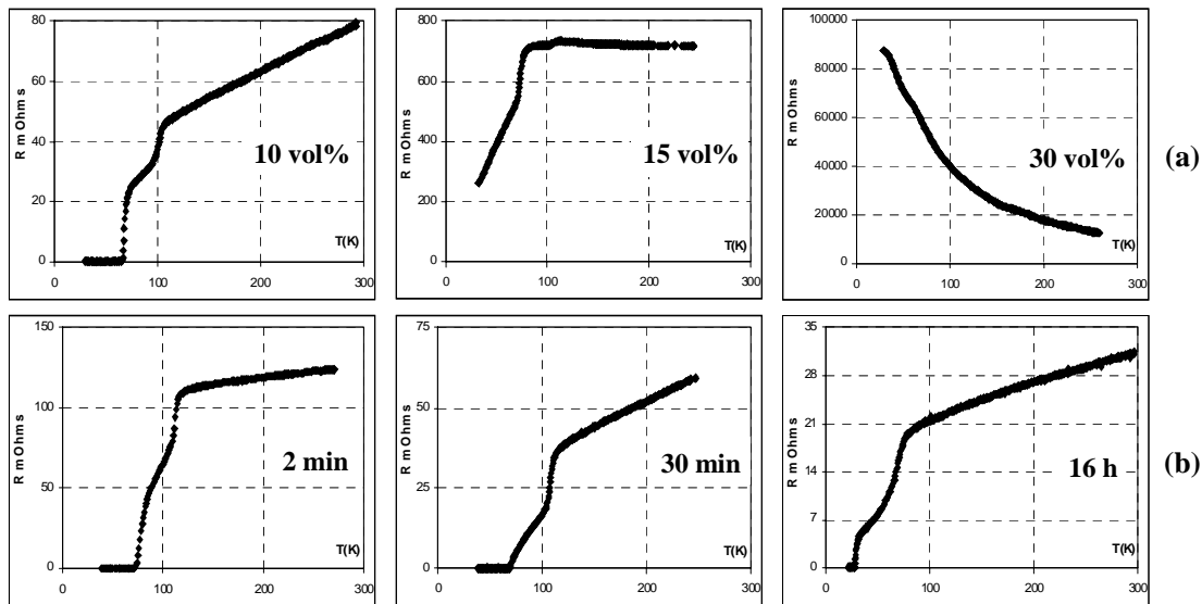
Fig. 1. R(T) plots for \text{In}_2\text{O}_3/\text{Bi-2223} depending on the vol% of \text{In}_2\text{O}_3 ( T_{\text{sintering}} = 830\text{ K} ; 16 hours) (a) and on the sintering duration for \text{In}_2\text{O}_3(2\text{ vol}\%) ( T_{\text{sintering}} = 830\text{ K} ) (b).
