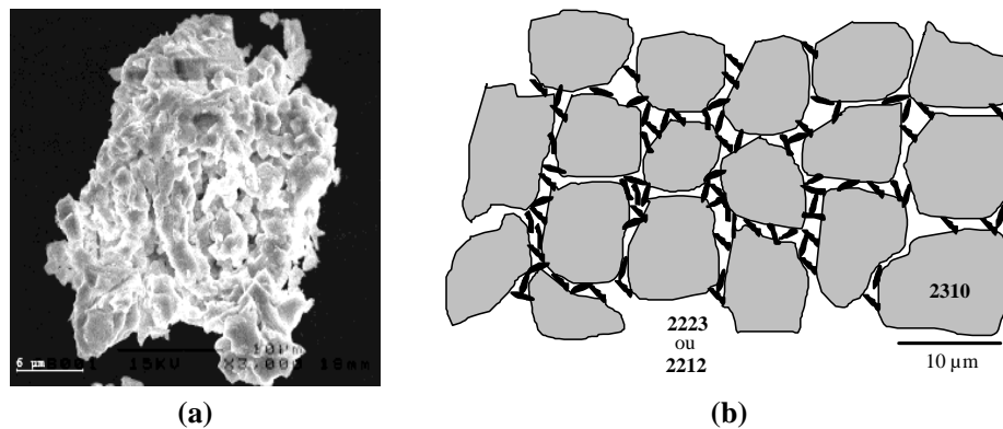
Fig. 2. SEM observations of \text{BiPb-2223}(20\%)/\text{Bi}_2\text{Sr}_3\text{CaO}_7 composite: picture of \text{Bi}_2\text{Sr}_3\text{CaO}_7 nodules heap (a) and schematic representation of the 3D network (b).
