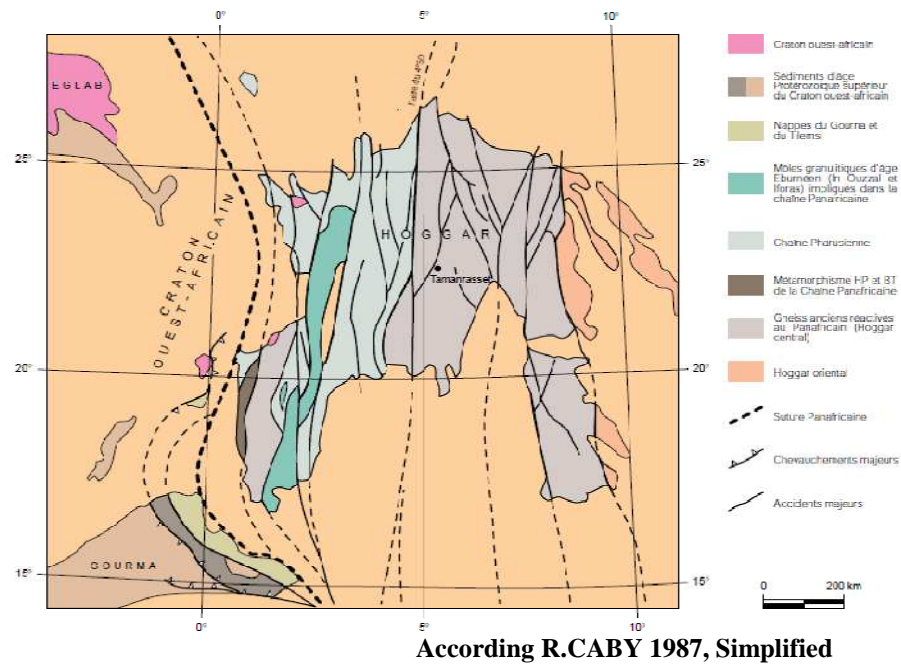
Figure 2: Simplified Geology of the Hoggar Shield
