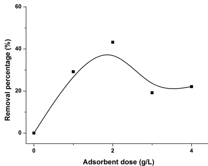
Fig. 11 – Effect of adsorbent (raw IMCM) dose on adsorption of NR dye.
