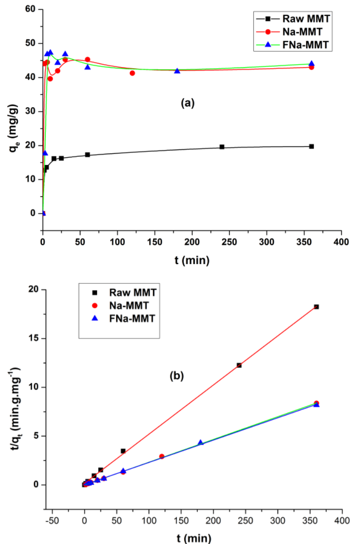
Fig. 7 – Adsorption kinetic of Nylosan Red onto inorganic clay materials (a), and pseudo second-order kinetics modeling (b).
