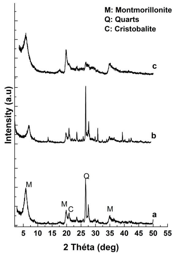
Fig. 1 – XRD patterns of raw IMCM a), Na-IMCM b) and FNa-IMCM c).
