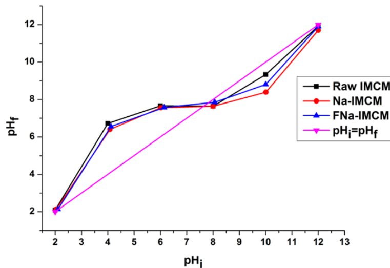
Fig. 5 – Evolution of the pH f according to the pH i of the samples.
