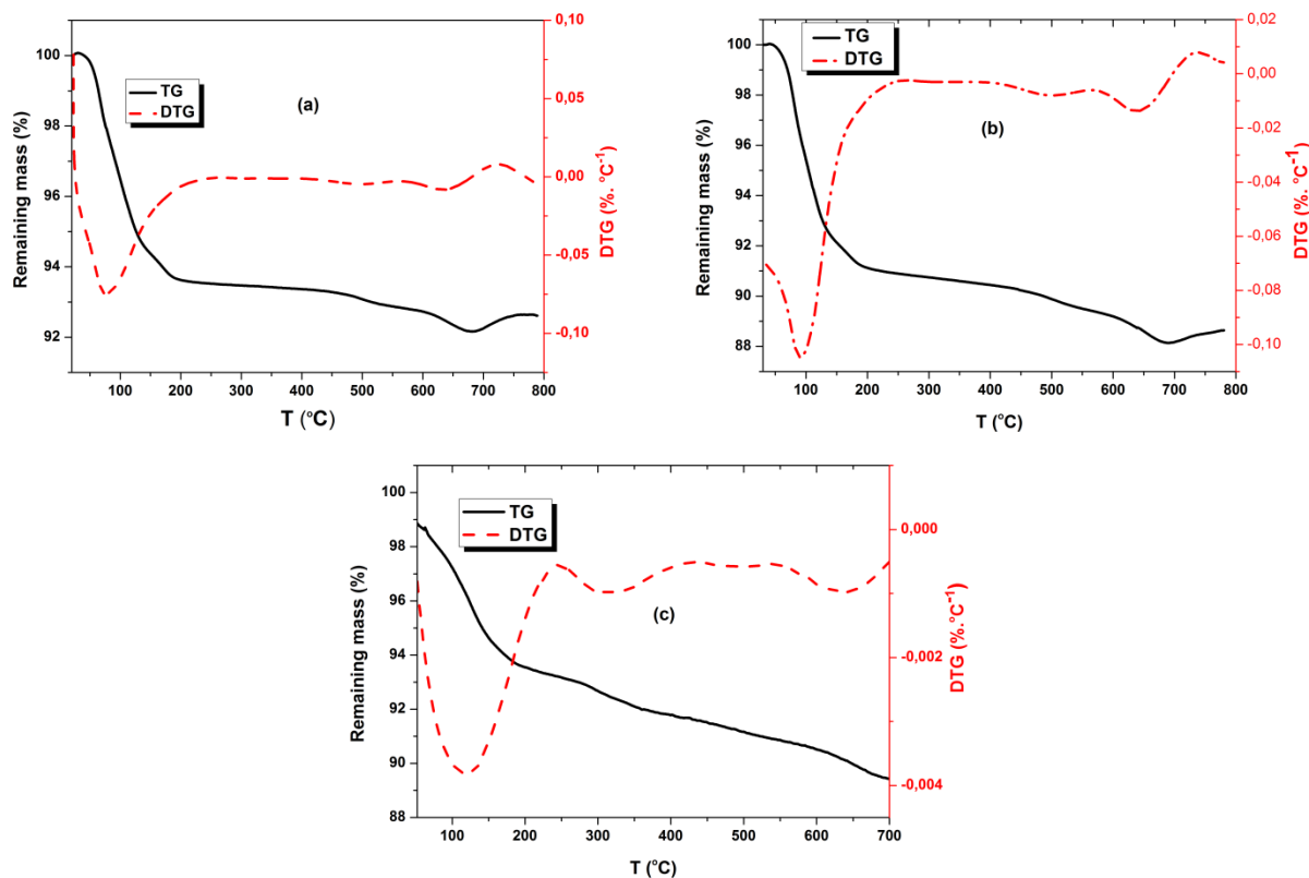
Fig. 3 – TG and DTG curves of raw IMCM a), Na-IMCM b) and FNa-IMCM ( 36 c).
