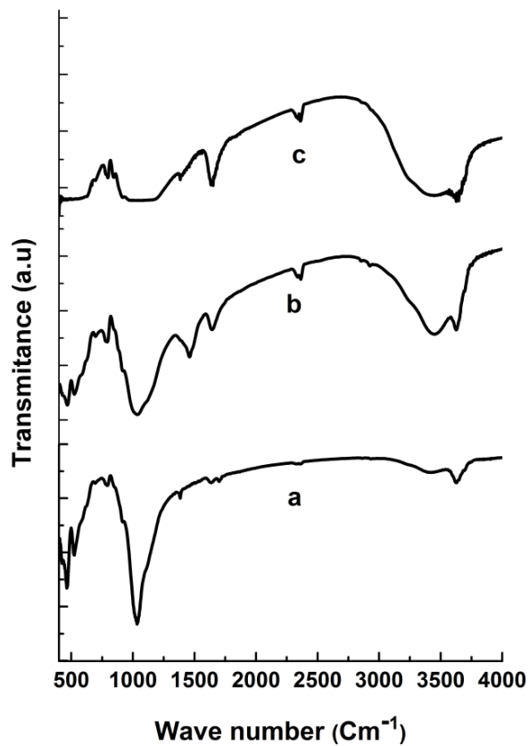
Fig. 2 – Infrared spectra of Raw IMCM a), Na-IMCM b) and FNa-IMCM c).
