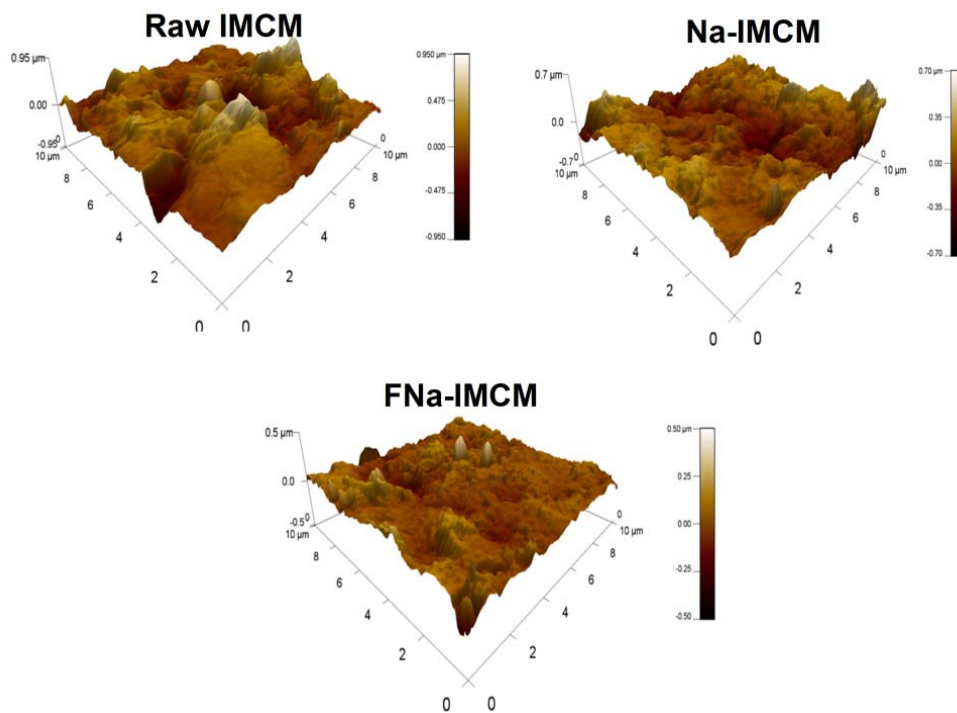
Fig. 4 – AFM images of raw IMCM (a), Na-IMCM (b) and FNa-IMCM ( 36 c).
