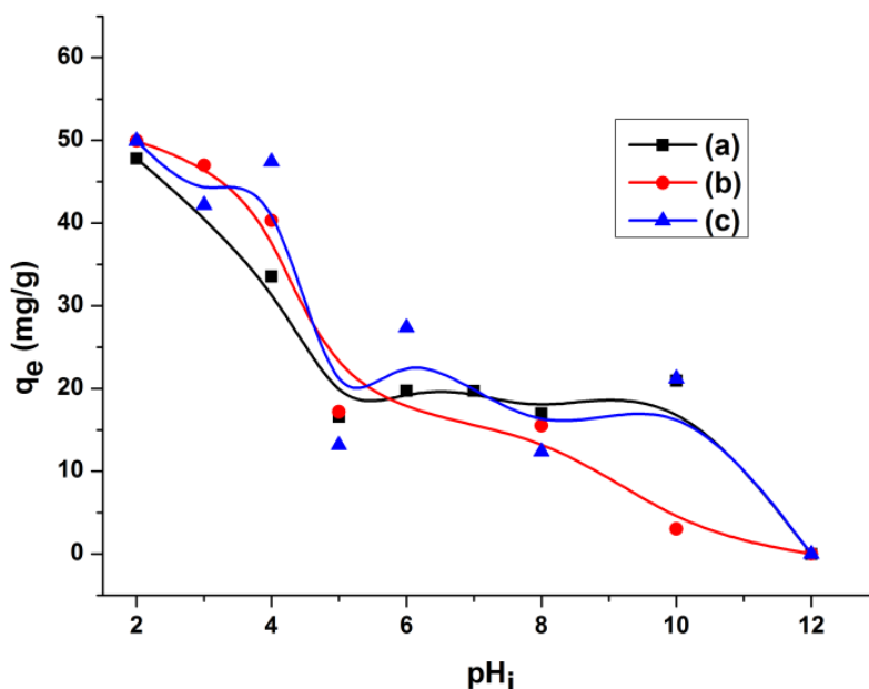
Fig. 6 – Effect of pH on adsorption of RN by raw IMCM a), Na-IMCM b) and FNa-IMCM c).
