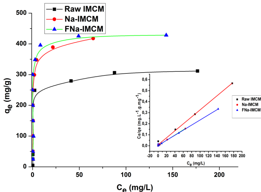
Fig. 10 – Equilibrium isotherms for adsorption of MB onto inorganic clay materials.
