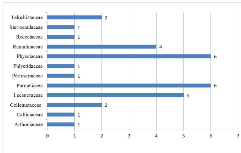
Fig. 6. Distribution of species by family (cedar section)
