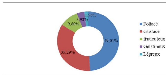
Fig. 5. Physiognomic appearance of the lichens inventoried
