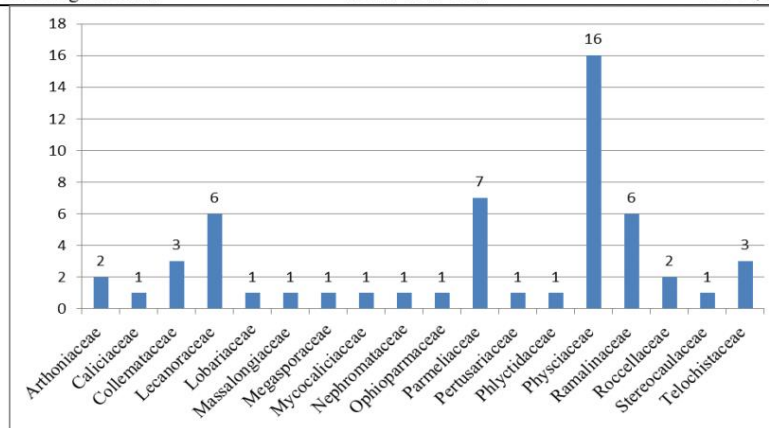
Fig. 4. Distribution of species according to families
