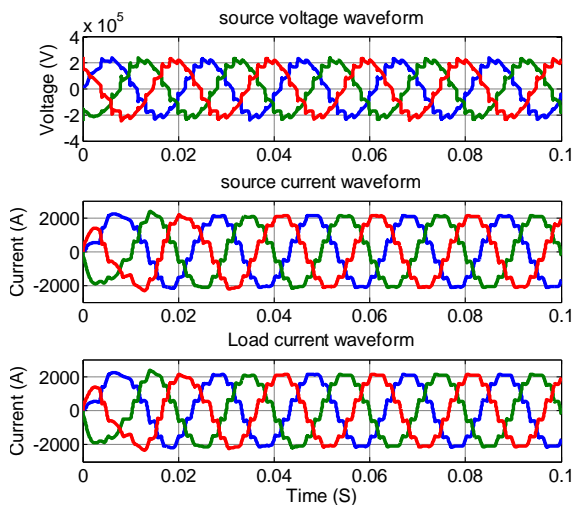
Fig.4. Voltages and currents in uncompensated HVDC system
