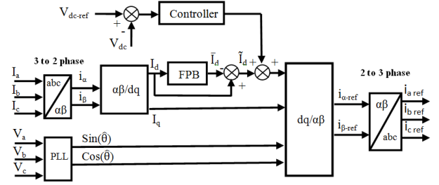
Fig.1. Synchronous reference frame theory
