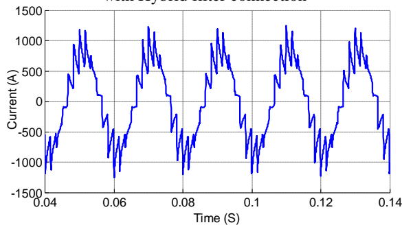
Fig.9. Active Filter injecting current i_{f1} (A)
