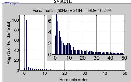
Fig. 5. Harmonics spectrum of source current without filter
