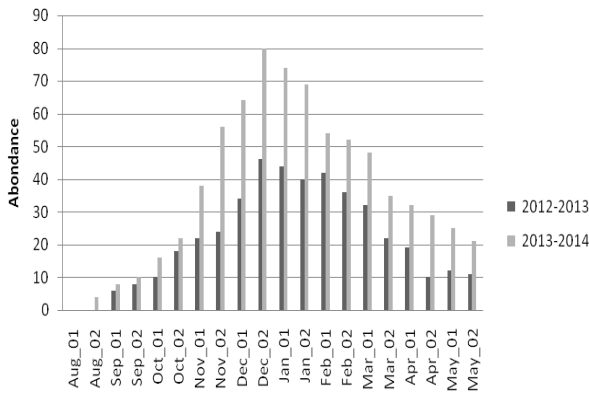
Figure 3. Seasonal changes in Ruddy Shelduck numbers on the lake Hamraia in 2012/2013 and 2013/2014.
