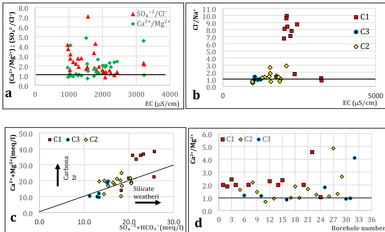
Fig. 11 Bivariate plots of a EC against (\text{Ca}^{2+}/\text{Mg}^{2+}) and (\text{SO}_4^{2-}/\text{Cl}^-) . b EC against (\text{Cl}^-/\text{Na}^+) vs. (\text{Under Na}^+ exchange reactions with \text{Ca}^{2+} and \text{Mg}^{2+} in clay layers). c (\text{SO}_4^{2-} + \text{HCO}_3^-) against (\text{Ca}^{2+} + \text{Mg}^{2+})
