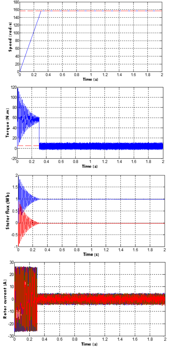
Figure 8. Type-2 fuzzy sliding mode control of the DFIM with rotor resistance variation
