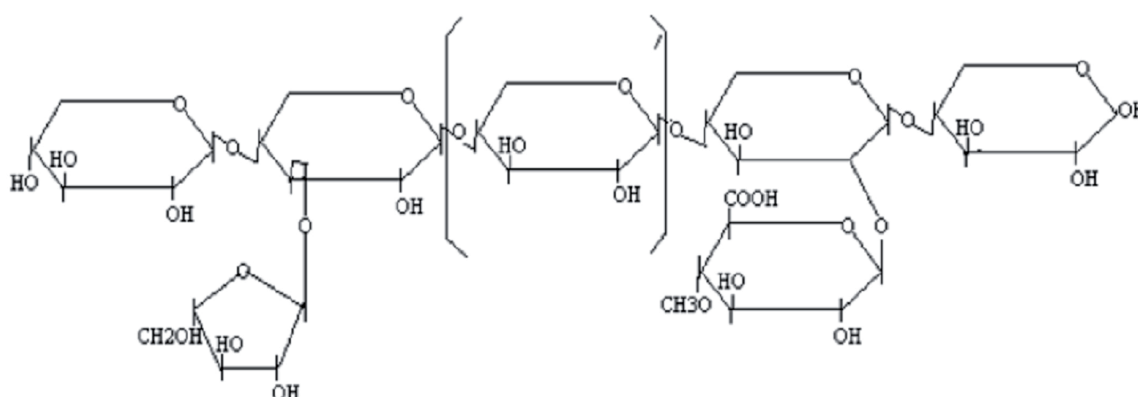
Figure 4. Structure of hemicellulose (1).
