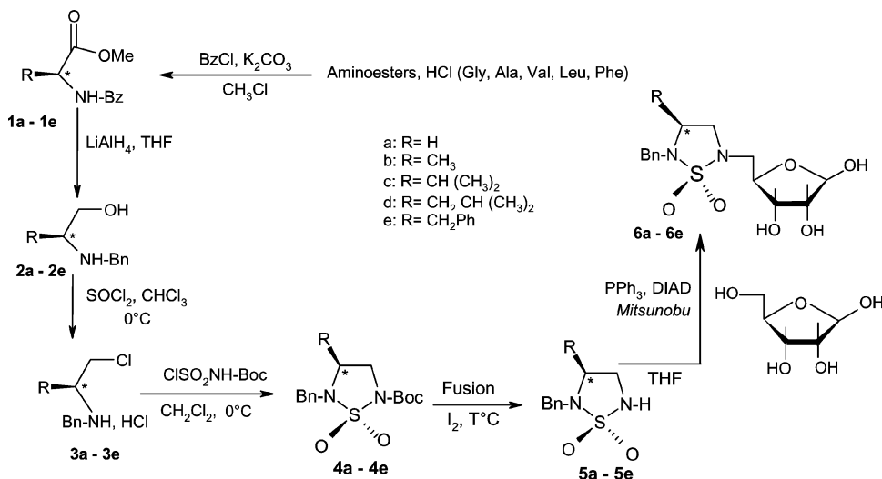
SCHEME 1 Synthesis of pseudonucleosides containing cyclosulfamide as aglycone (5-deoxy-5-(5-2-benzyl-3(S)-alkylthiadiazolidinyl)- \beta -D-ribose).
