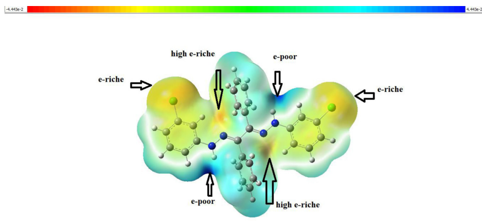
Fig. 9. Molecular electrostatic potential map of 3-Cl BHB.
