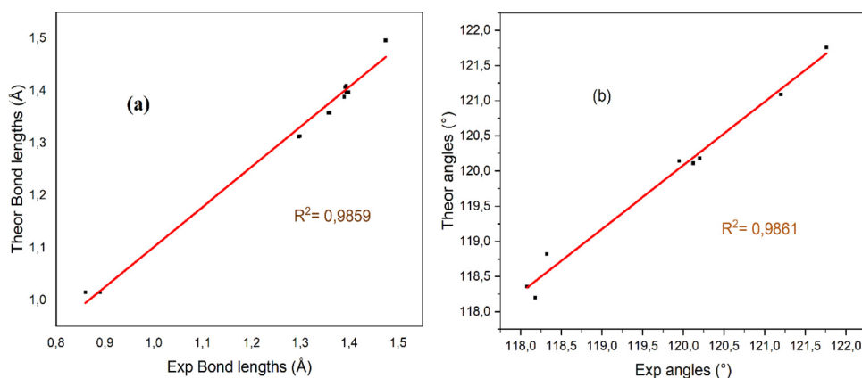
Fig. 7. DFT/XRD-graphical correlation for bond lengths (a) and bond angles (b).
