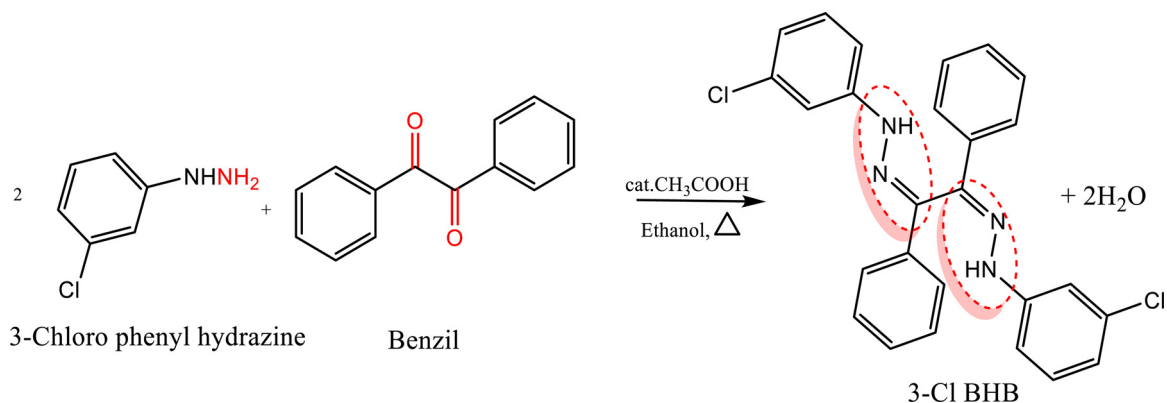
Scheme 1. The synthesis schematic for (1Z,2Z)-1,2-bis (3-Chlorophenyl Hydrazino) Benzil.
