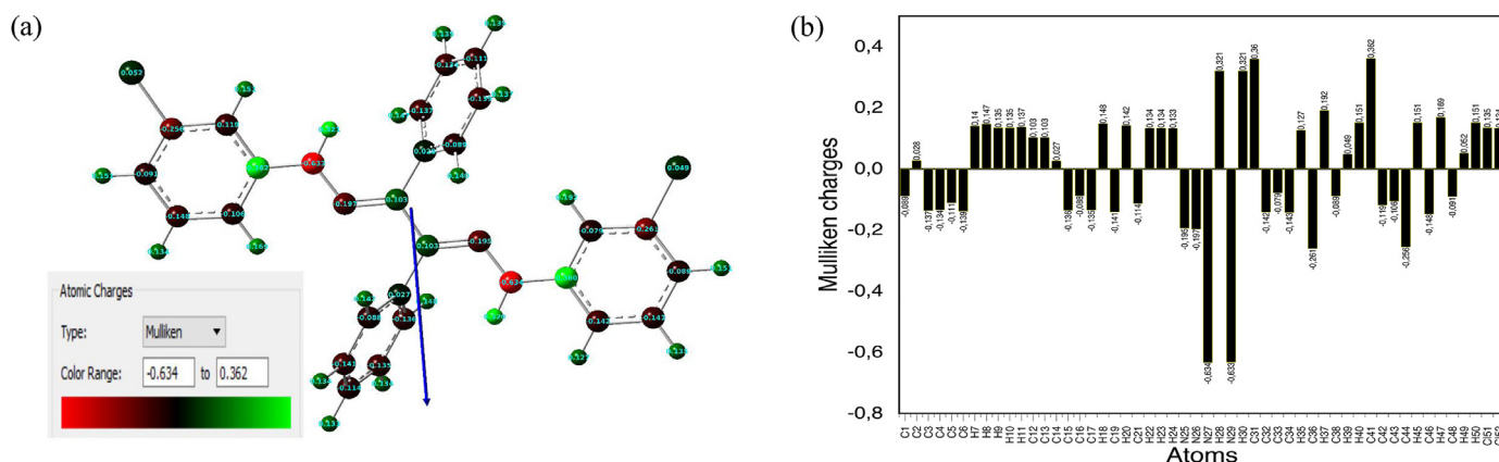
Fig. 10. (a). Mulliken atomic charges of 3-Cl BHB calculated at B3LYP/6-31 G (d,p) level. (b). The Mulliken atomic charge distribution of 3-Cl BHB.
