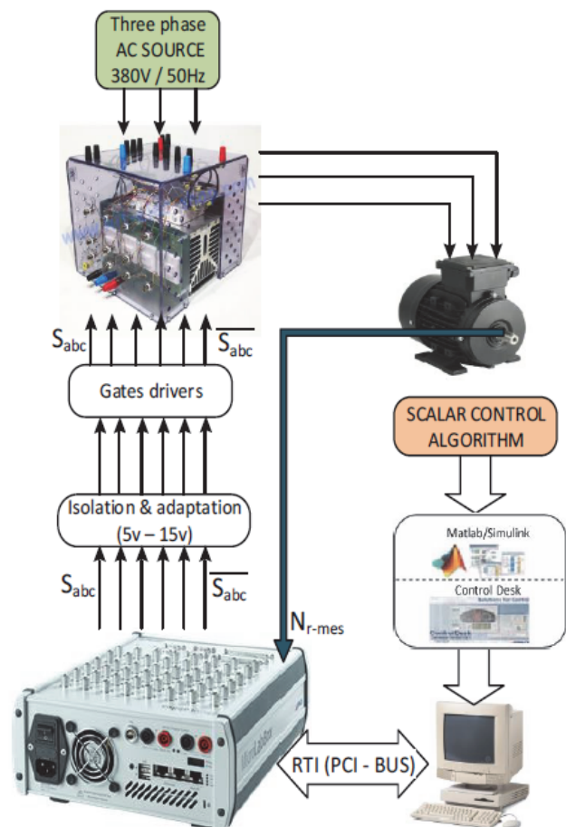
Fig. 1. Basic scalar control schema.
