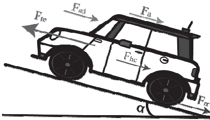
Fig. 5. Types of forces applied to the vehicle.
