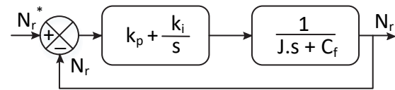
Fig. 3. Speed regulation.
