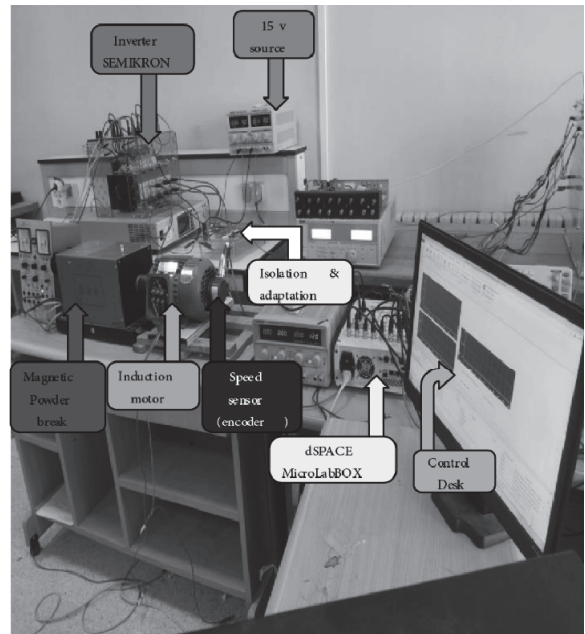
Fig. 6. Experiment prototype for laboratory
