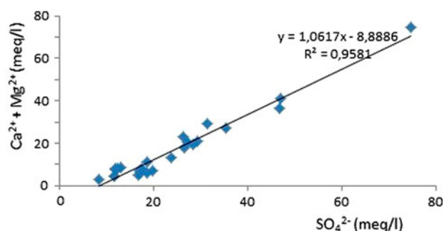
Fig. 5. Relationship \text{Ca}^{2+} + \text{Mg}^{2+} vs. \text{SO}_4^{2-} in groundwater Chemora.
