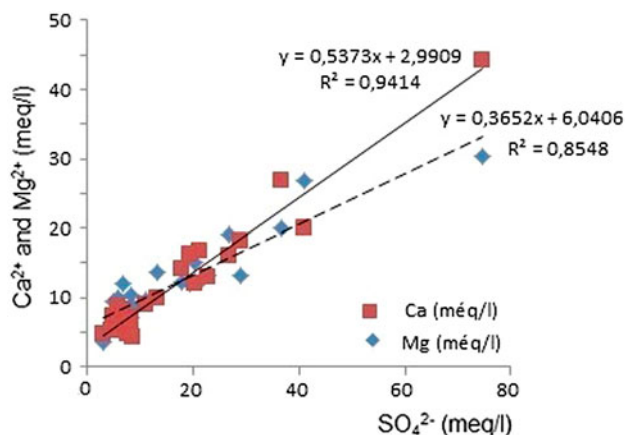
Fig. 3. Relationship \text{Ca}^{2+} , \text{Mg}^{2+} vs. \text{SO}_4^{2-} in groundwater Chemora.
