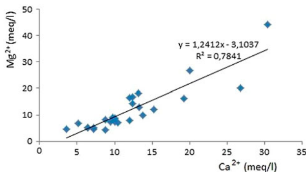
Fig. 4. Relationship \text{Ca}^{2+} vs. \text{Mg}^{2+} in groundwater Chemora.
