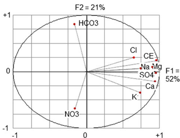
Fig. 9. Factorial plane F1–F2.
