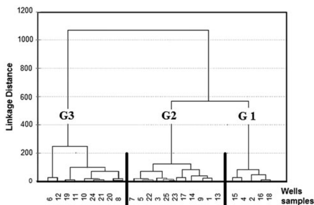
Fig. 8. Cluster dendrogram for water samples.
