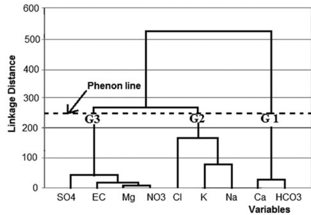
Fig. 7. Cluster dendrogram for variables.
