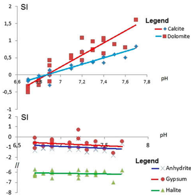
Fig. 6. Variation of the saturation index of carbonate minerals in the groundwater of Chemora.
