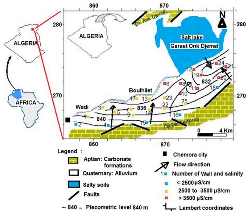
Fig. 1. Hydrogeological map of the study area.
