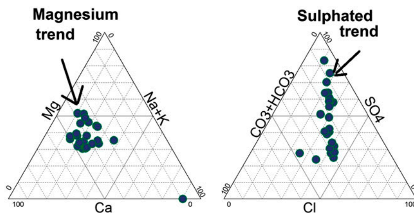
Fig. 2. Piper diagram Piper applied to Chemora groundwater.
