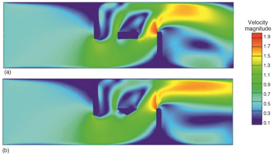
Figure 5. Mean velocity fields in both studied cases, Re = 5000 ; (a) baffled channel with a rectangular turbulator and (b) baffled channel with a triangular turbulator
