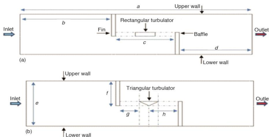
Figure 1. Schematic diagram of the baffled heat exchanger channel, in both turbulator cases; (a) rectangular and (b) triangular
