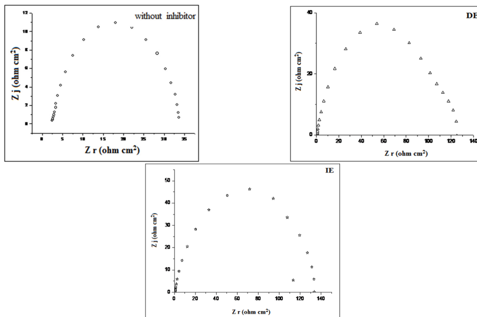
Figure 13. Nyquist diagrams for mild steel in 1M HCl acid solution without and with presence of aqueous extracts at 180 mg/L
