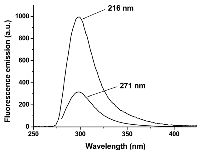
Fig. 6 Fluorescence spectra of Tramadol 0.01 mmol·L -1 for excitation wavelengths of 216 nm and 271 nm
