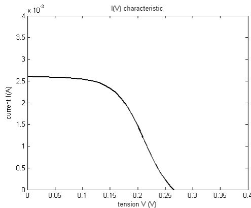
Fig.9: I(V) characteristic for the MPP/ZnPc structure.
