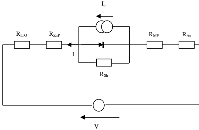
Fig. 8: Electric circuit of the MPP/ZnPc cell [23].
