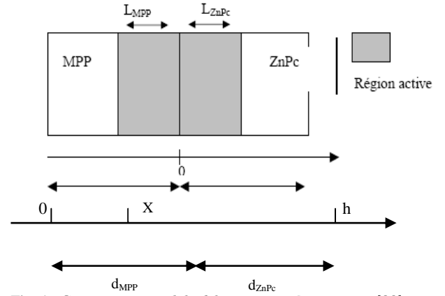
Fig. 4 : Geometrical model of the MPP/ZnPc structure [23].
