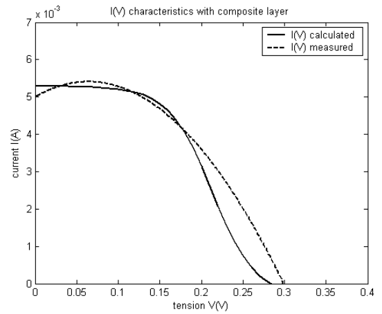
Fig. 10 : I(V) characteristic for the MPP/ZnPc structure containing the composite layer ZnPc/C 60 (1:1).
