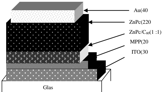
Fig. 3: Structure of the substrat/ITO/MPP/ZnPc/Au cell [23].
