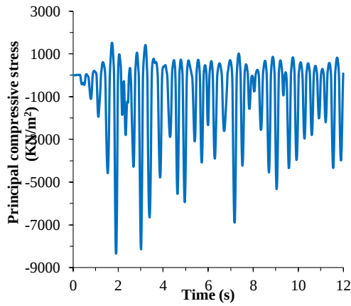
a) linear analysis
