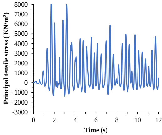
a) linear analysis
