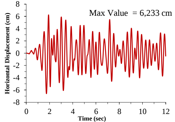
b) Nonlinear analysis
