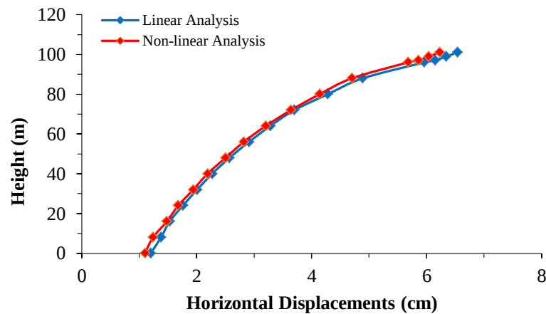
Figure 4 Maximum horizontal displacements in upstream direction according to linear and nonlinear analyses
