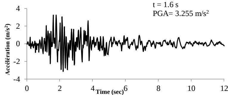
Figure 3 Time history of horizontal acceleration for 1980 El Asnam earthquake record scaled by factor of 2.5
