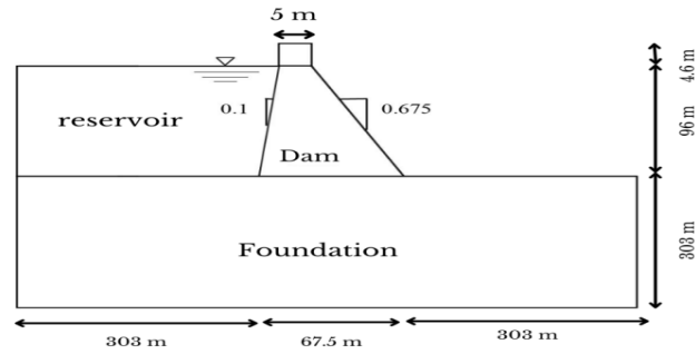
Figure 1 Transverse Section and Dimensions.
