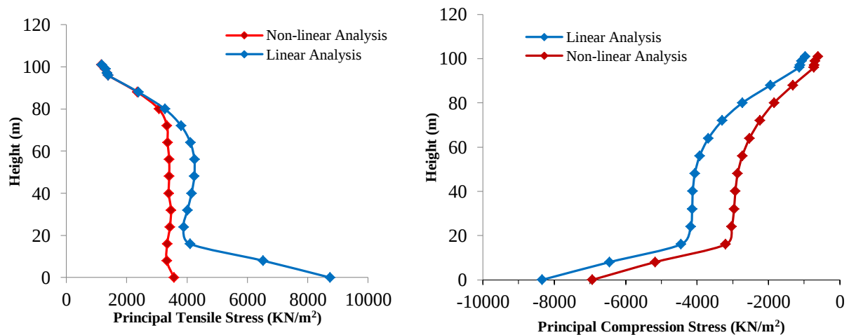
Figure 6 Maximum principal stresses along dam height according to linear and nonlinear analyses
