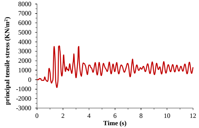
b) Nonlinear analysis
