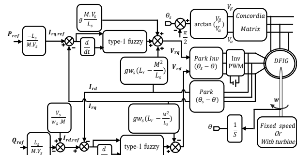
Fig.3. Block diagram of the type 1 fuzzy logic control structure
