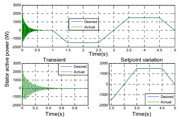
Fig.9. Stator active power
