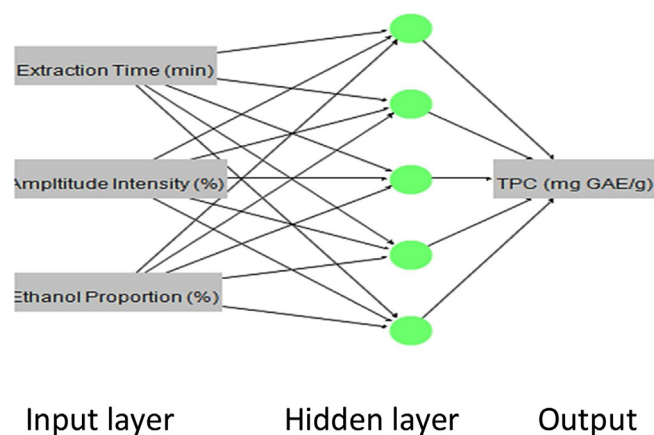
Fig. 1. ANN design for three operating parameters (irradiation time (X 1 ); Amplitude (X 2 ) and ethanol proportion (X 3 )) as input, and TPC yield as output.
