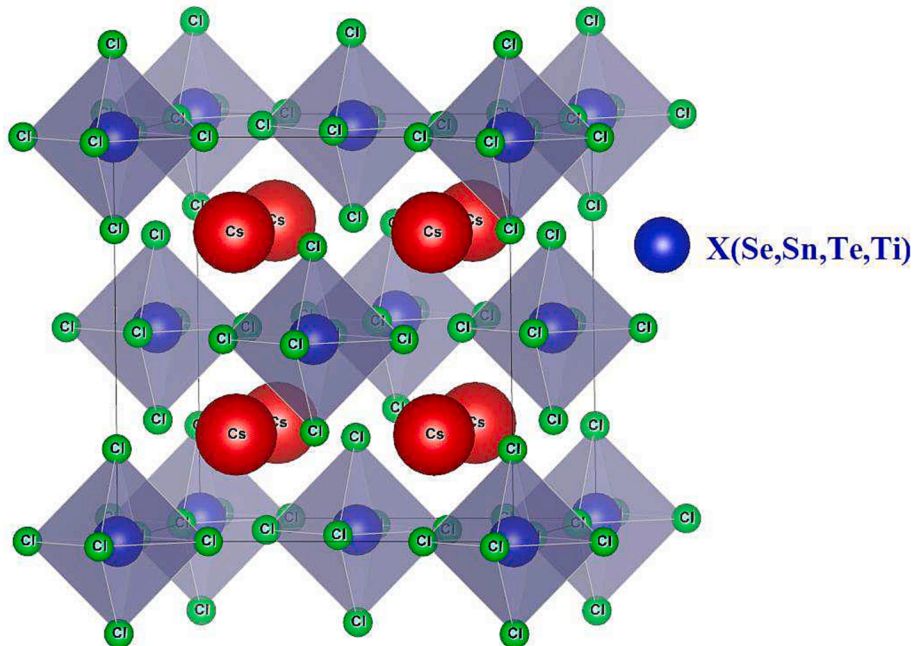
Fig. 1. The crystal structure of Cs_2XCl_6 ( X = Sn, Se, Te and Ti ) double perovskites.
