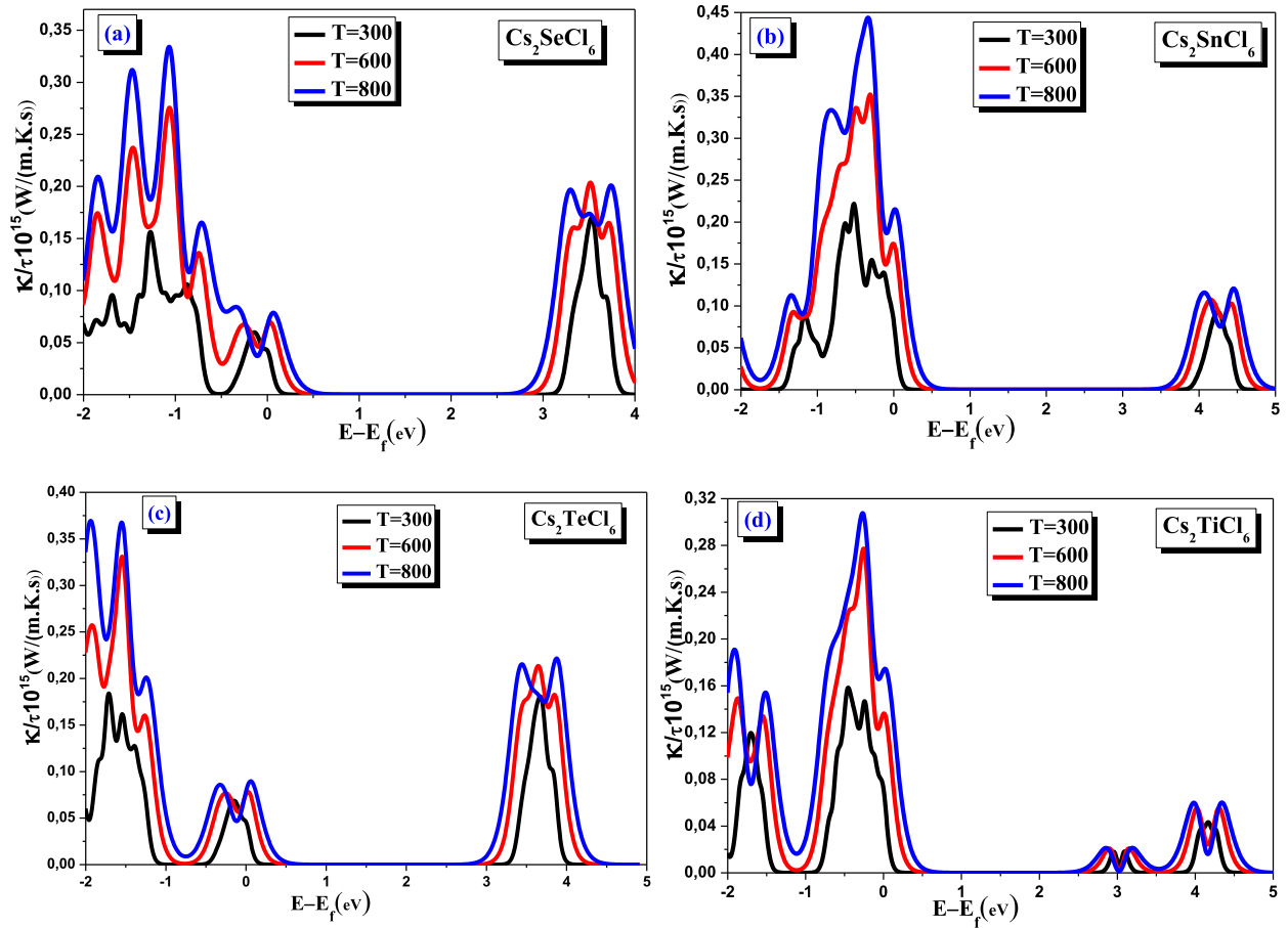
Fig. 11. Electronic thermal conductivity as a function of chemical potential at temperatures T = 300 K, 600 K and 800 K for (a) \text{Cs}_2\text{SeCl}_6 , (b) \text{Cs}_2\text{SnCl}_6 , (c) \text{Cs}_2\text{TeCl}_6 and (d) \text{Cs}_2\text{TiCl}_6 using GGA-mBJ.
