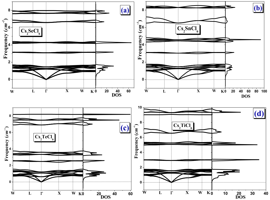
Fig. 4. Phonon band structures and DOS of \text{Cs}_2\text{XCl}_6 ( X = \text{Se}, \text{Sn}, \text{Te} and \text{Ti} ) using GGA-mBJ.
