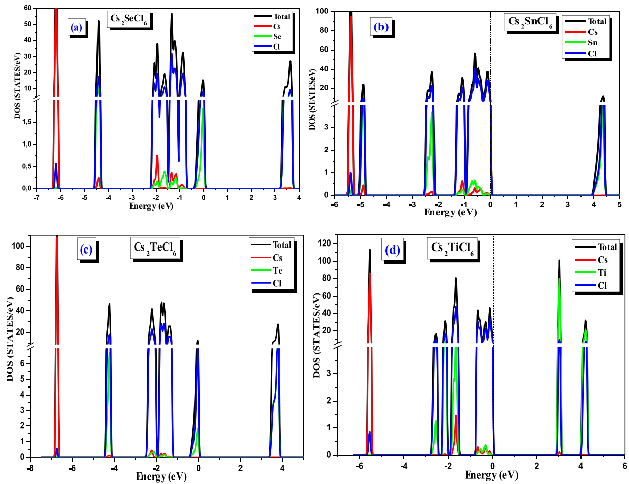
Fig. 7. The density of states of \text{Cs}_2\text{MCl}_6 ( \text{M} = \text{Se}, \text{Sn}, \text{Te} and \text{Ti} ) using GGA-mBJ.
