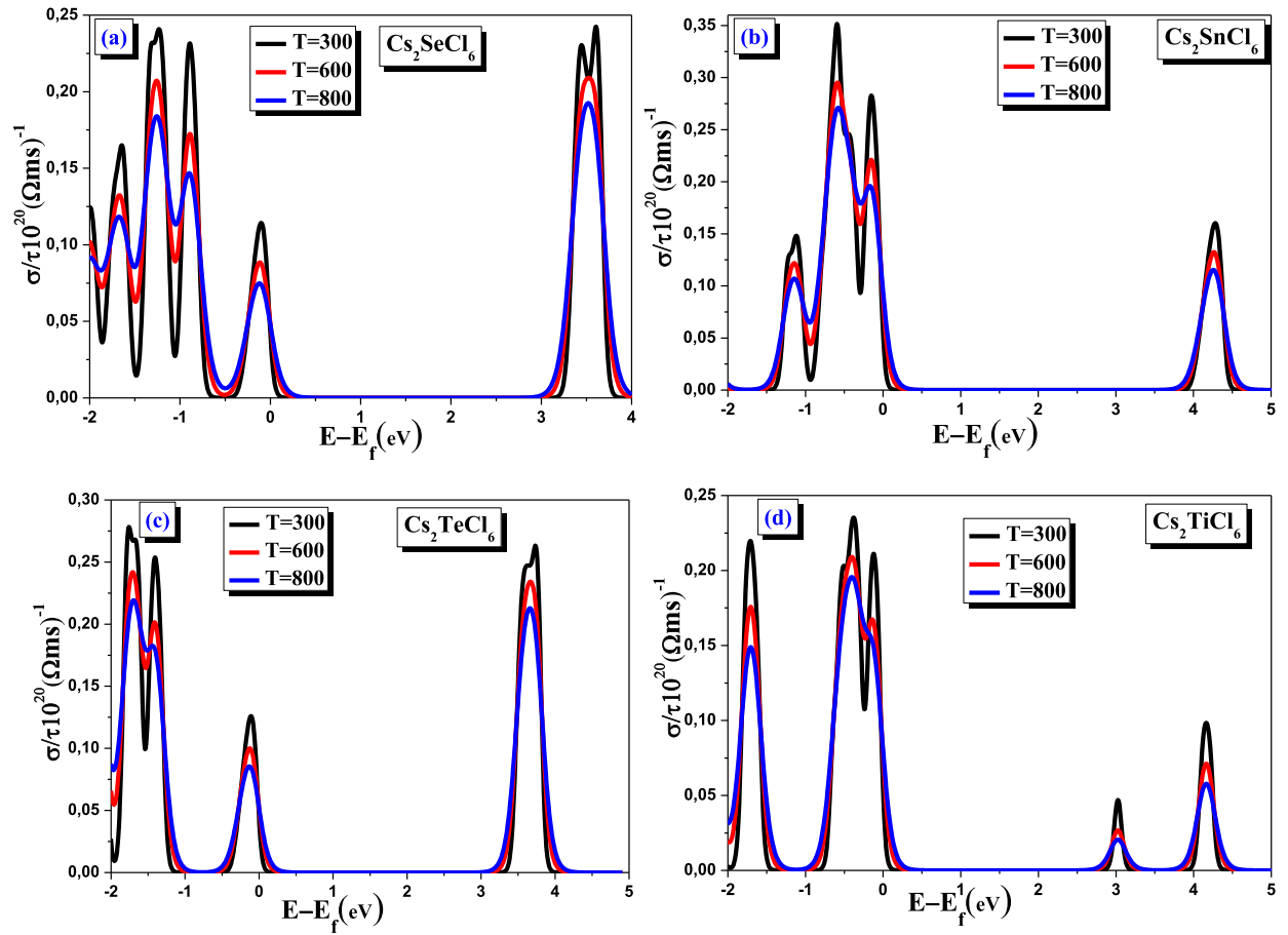
Fig. 10. Electrical conductivity as a function of chemical potential at temperatures T = 300 \text{ K} , 600 \text{ K} and 800 \text{ K} for (a) \text{Cs}_2\text{SeCl}_6 , (b) \text{Cs}_2\text{SnCl}_6 , (c) \text{Cs}_2\text{TeCl}_6 and (d) \text{Cs}_2\text{TiCl}_6 using GGA-mBJ.
