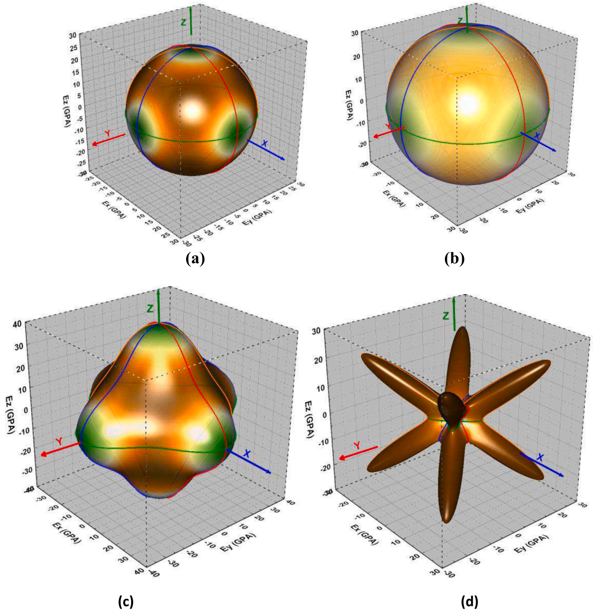
Fig. 5. The 3D surface construction of Young's modulus in \text{Cs}_2\text{SeCl}_6 (a), \text{Cs}_2\text{SnCl}_6 (b), \text{Cs}_2\text{TeCl}_6 (c) and \text{Cs}_2\text{TiCl}_6 (d) using GGA.
