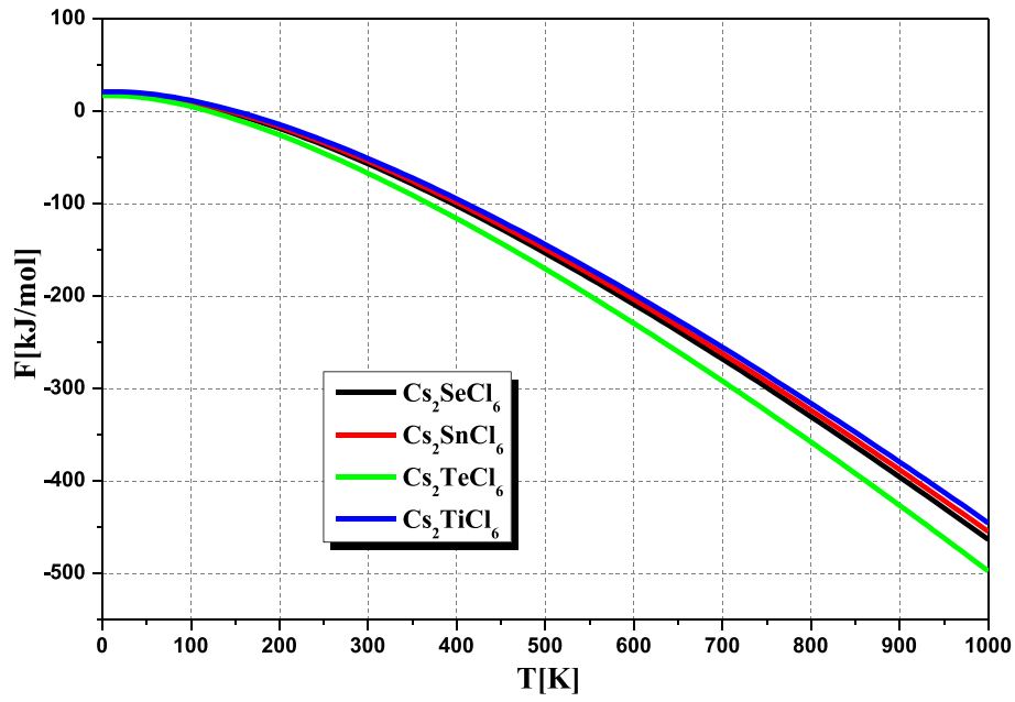
Fig. 3. Helmholtz free energy of \text{Cs}_2\text{XCl}_6 ( X = \text{Se}, \text{Sn}, \text{Te} and \text{Ti} ) as a function of temperature.
