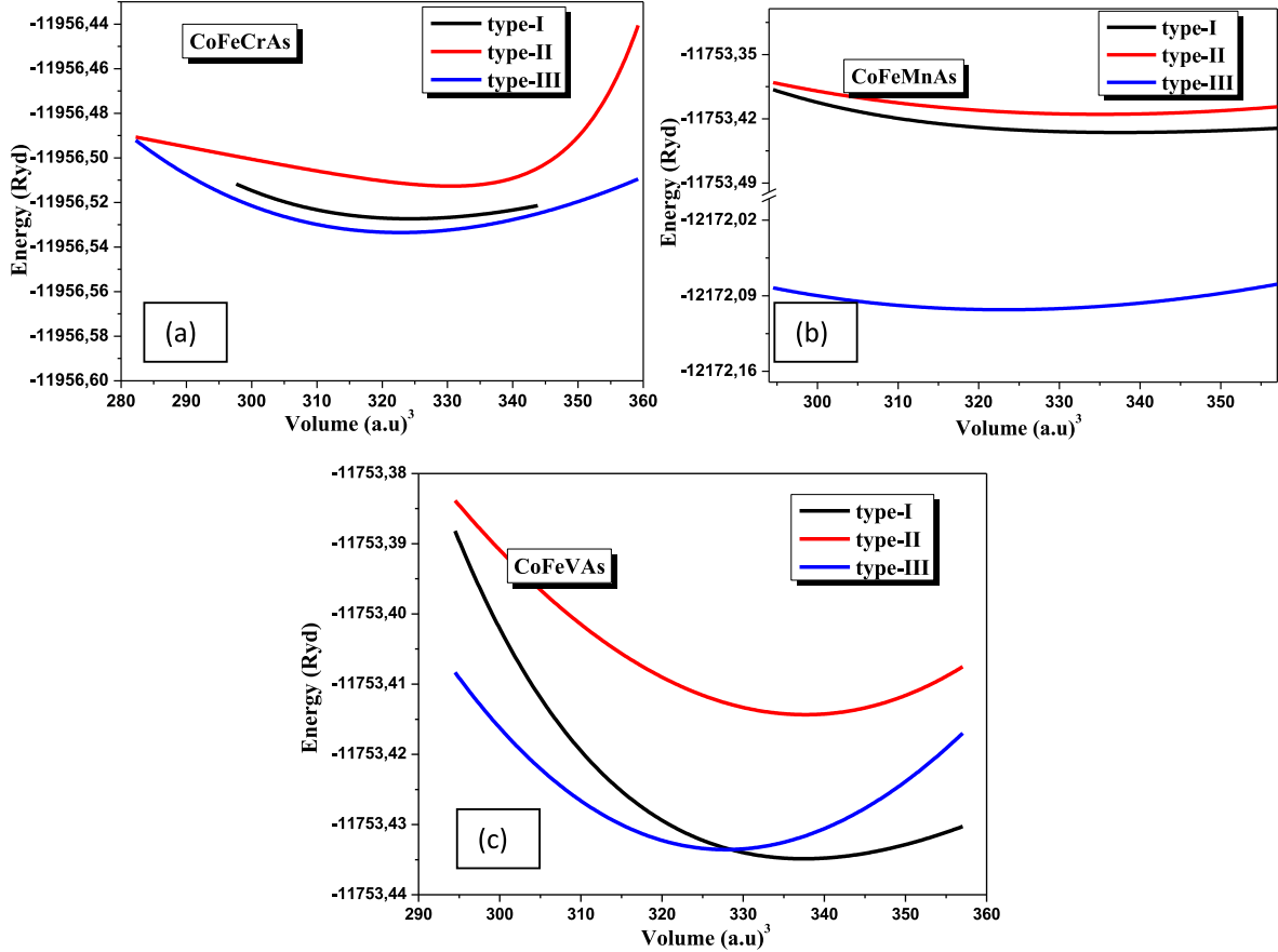
Fig. 2. Energy change with respect to volume for (a) \text{CoFeCrAs} , (b) \text{CoFeMnAs} and (c) \text{CoFeVAs} in the ferromagnetic phase.
