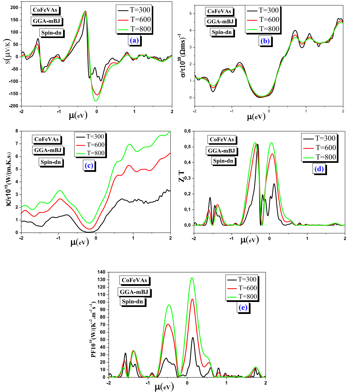
Fig. 14. The Seebeck coefficient (a), electrical conductivity (b), electronic thermal conductivity (c), figure of merit (d), and power factor (e) as a function of chemical potential for CoFeVAs spin dn.
