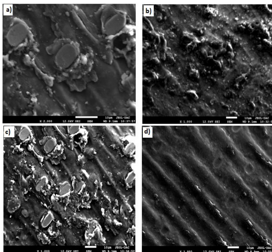
Figure 7: SEM micrographs of untreated and treated composites; (a) UTAF, (b) ATAF31, (c) ATAF33, (d) ATAF35
