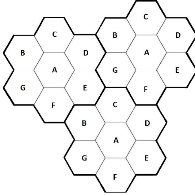
Figure I.3: Example of frequency reuse[22].
