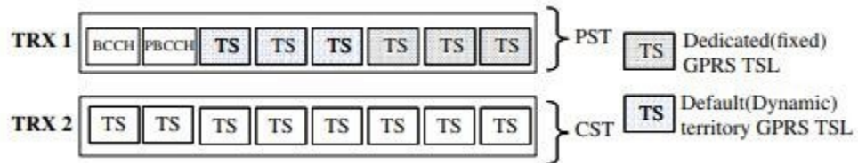
Figure I.4: GPRS timeslot allocation to CS and PS traffic[17].
