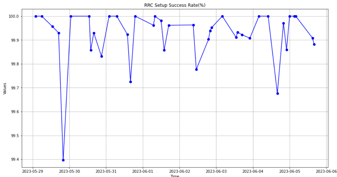
Figure IV.4: KPI RRC Setup success rate (%) in the cell 283004.
