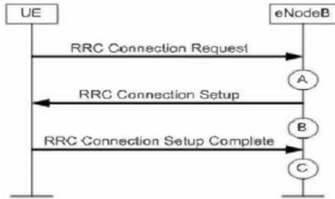
Figure II.4: Measurement point for RRC connection setup[11].
