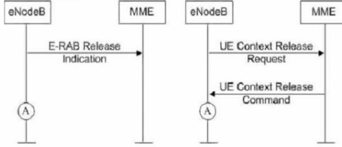
Figure II.7: Abnormal ERAB release[22].
