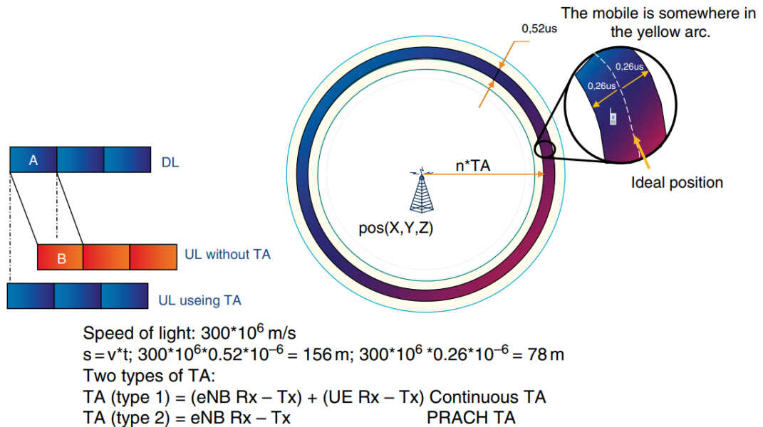
Figure III.6: Timing Advance in LTE[22].
