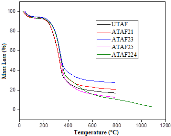
Figure3 TGA of untreated and NaOH-treated Alfa fibers at different times(1,3,5 and 24 h)
