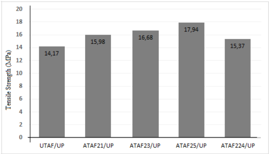
Figure 5 Effect of chemical treatment time on the tensile strength of the studied composite
