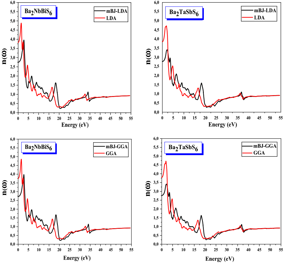
Fig. 9. (Color online) Variation of refractive index as a function of photon energy for the compounds Ba_2NbBiS_6 and Ba_2TaSbS_6 with the GGA, mBJ-GGA, LDA and mBJ-LDA approximations.
