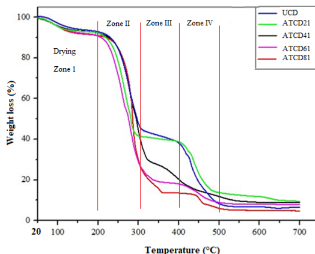
Figure 5: TGA curves of raw material and NaOH-treated Cynodon dactylon root-derived fibers at different concentrations (2, 4, 6 and 8%)
