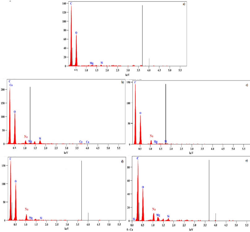
Figure 4: EDX spectra of (a) UCD; (b) ATCD21; (c) ATCD41; (d) ATCD61; (e) ATCD81
