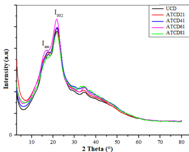
Figure 1: X-ray diffraction patterns of untreated and alkali-treated Cynodon dactylon root-derived fibers
