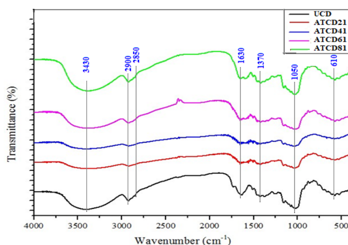
Figure 2: Infrared spectra of initial material and alkali-treated Cynodon dactylon fibers
