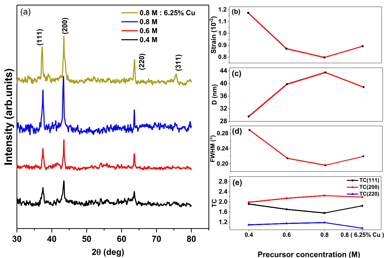
Fig. 2 (a) XRD Patterns, (b) strain variation, (c) crystallite size variation, (d) FWHM variation and (e) TC ( hkl ) variation of NiO thin films and CNO thin films (0.4 M, 0.6 M, 0.8 M, and 0.8 M with 6.25% Cu)
