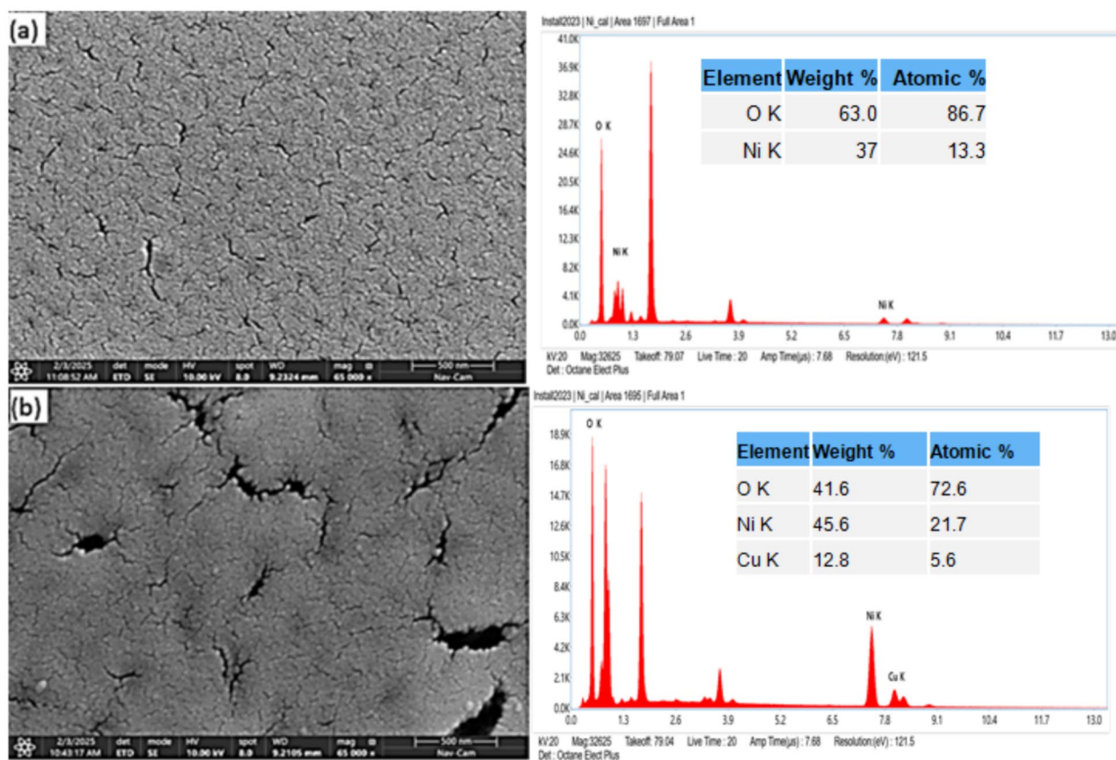
Fig. 4 SEM images and EDX spectra of (a) NiO (0.8 M) and (b) CNO thin films (0.8 M; 6.25% Cu). Accelerating voltage: 10.000 kV, Magnification: 65 000 x, Working distance for SEM: 9.2105 mm, Calibration standards used for EDS analysis: Fe
