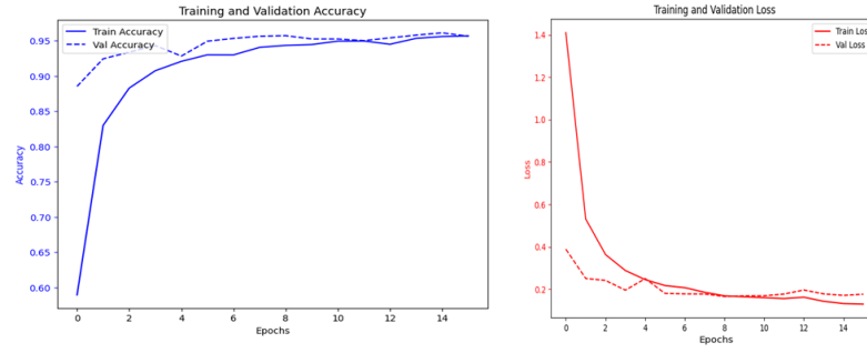
FIGURE 4. Training and Validation Accuracy and Loss Curves
