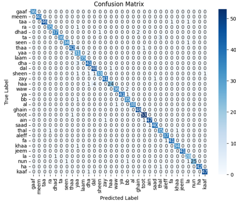
FIGURE 5. Confusion Matrice for ArSL using ResNet50
