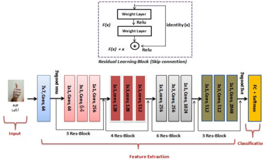
FIGURE 3. ResNet-50 Architecture with Residual Connections
