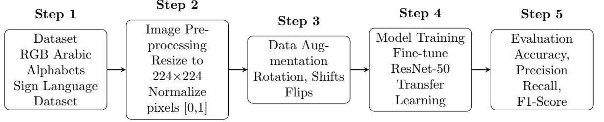
FIGURE 2. Horizontal Methodology Pipeline for Arabic Sign Language Recognition
