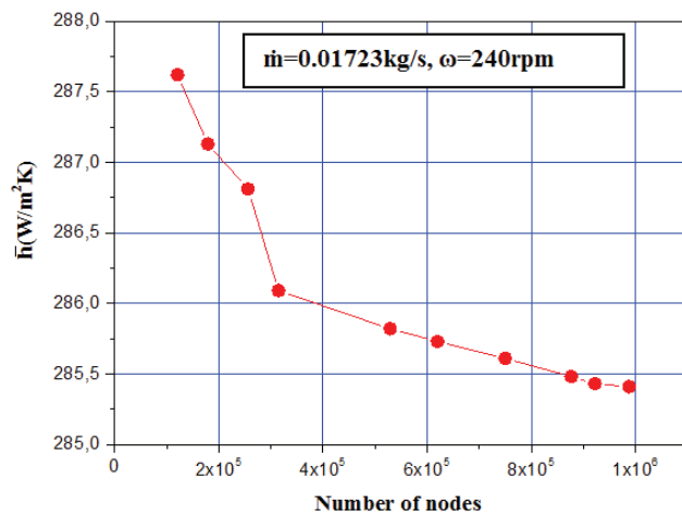
Figure 6. Variation of average convective heat transfer coefficient as a function of the number of nodes for \dot{m} = 0.01723 \text{ Kg/s} and \omega = 240 \text{ rpm} .
